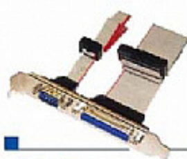
KF0507 AT/IO Mouse Cable | 10p IDC Socket to D-Sub 9p (M) +25p IDC Socket to D-Sub 25p (F) W/Bracket .
