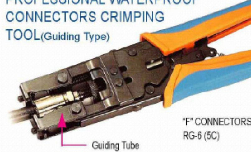
Adjustable Max. 10mm Interchangeable "F" (BNC,RCA)
