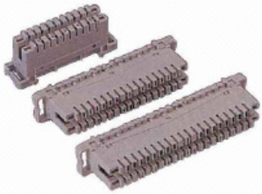
CM-10A 10 Pair Connection Modules Dimensions: 123.3 x 21.3 x 39.5mm
