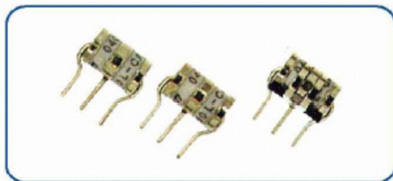
G-03001 Gas tube arrester. 3pole 350V w/o failsafe (7.5mm x 12mm)
