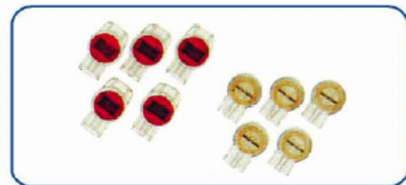
S-00006 Splicing UR connector. insulation: 1.67mm, conductor:0.4-0.9mm
